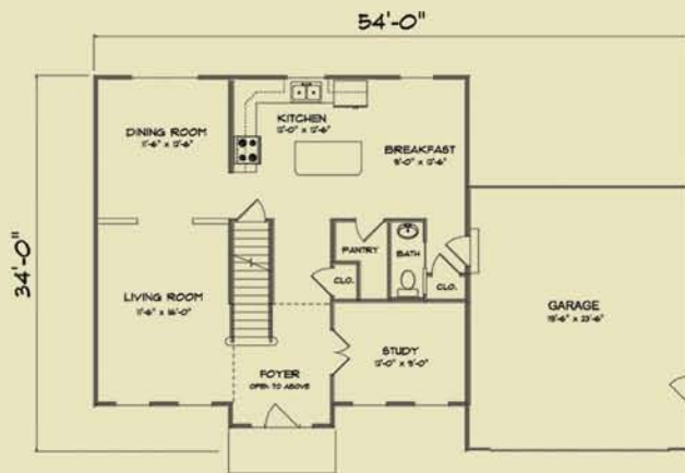
FIRST FLOOR 1040 SQUARE FEET
