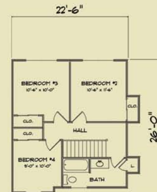
SECOND FLOOR 594 SQUARE FEET
