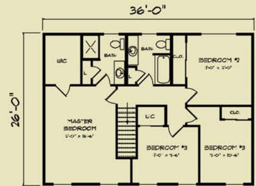
SECOND FLOOR 936 SQUARE FEET
