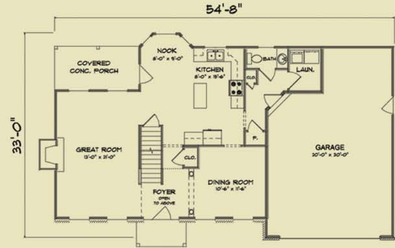
FIRST FLOOR 973 SQUARE FEET
