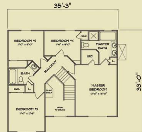
SECOND FLOOR 932 SQUARE FEET
