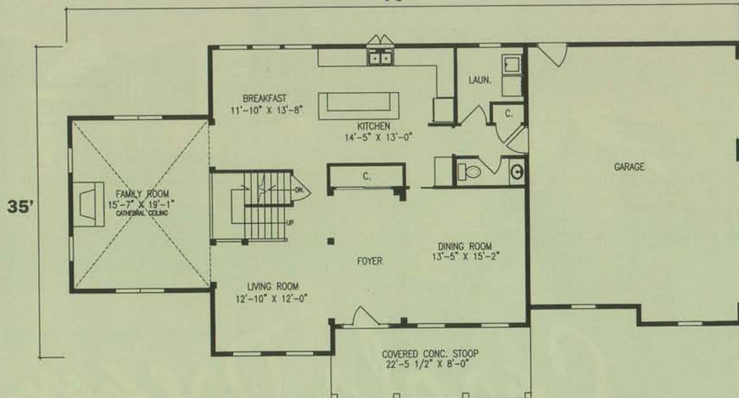
First Floor 1505 Square Feet
