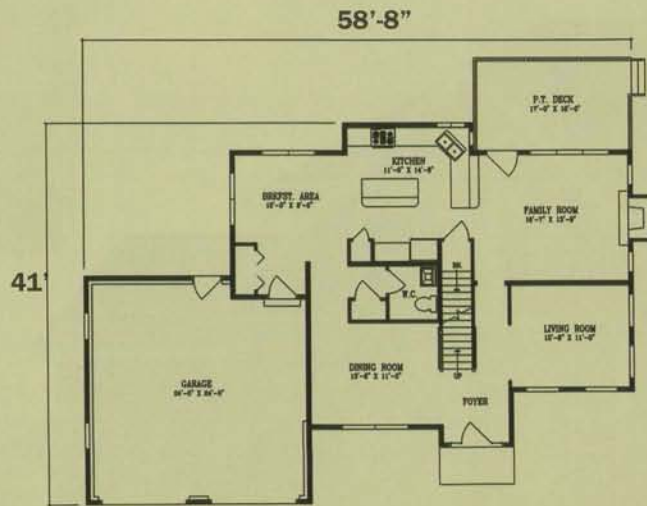
First Floor 1185 Square Feet
