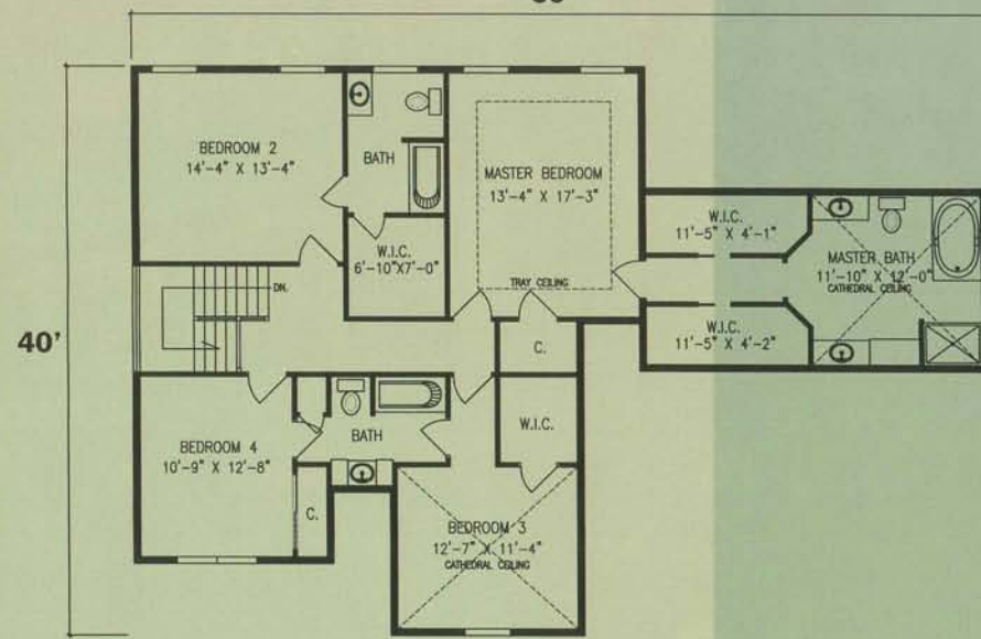
Second Floor 1544 Square Feet
