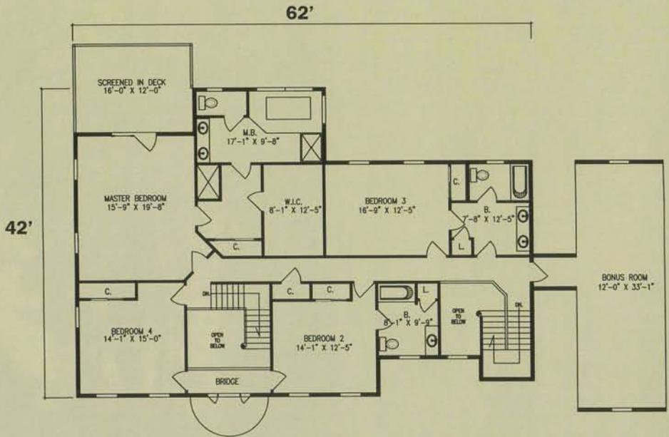
Second Floor 2574 Square Feet
