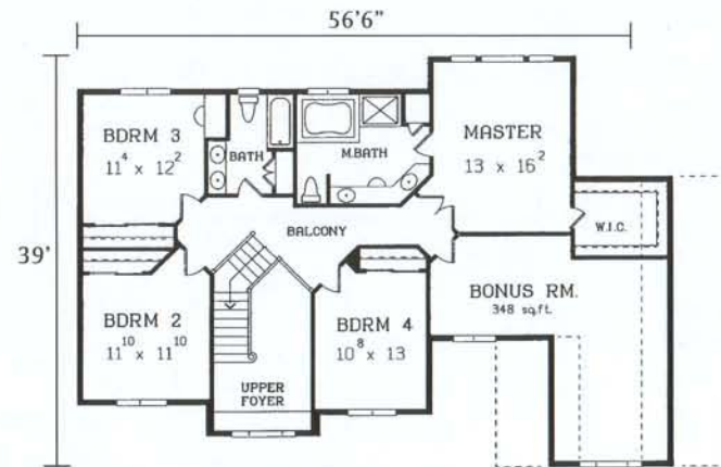
Second Floor 1563 Square Feet
