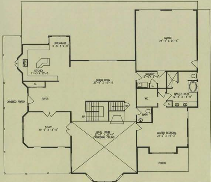
First Floor 3153 Square Feet
