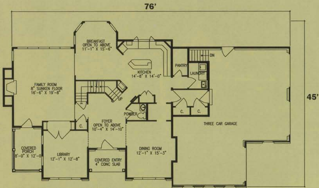
First Floor 1670 Square Feet
