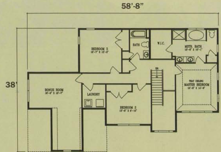
Second Floor 1425 Square Feet
