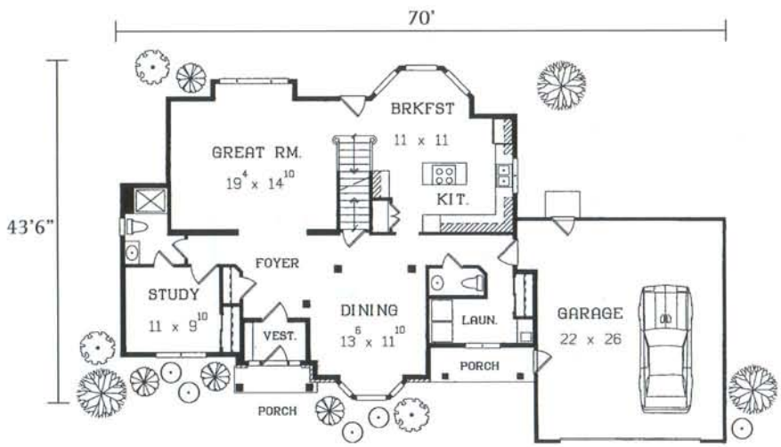
First Floor 1433 Square Feet
