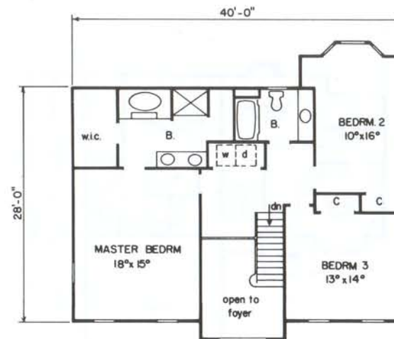
Second Floor 1115 Sq. Ft.
