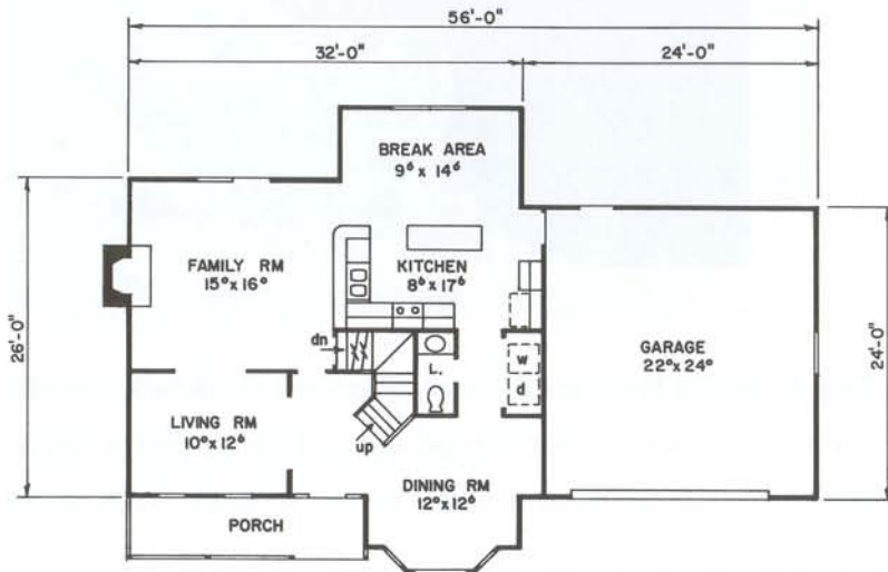
First Floor 1029 Sq. Ft.
