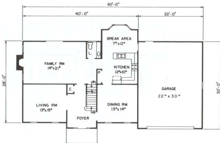
First Floor 1205 Sq. Ft.
