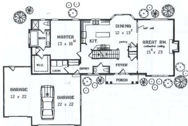
Harris Hideaway 2276 Square Feet
