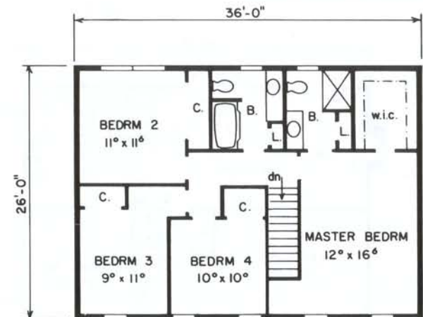
Second Floor 936 Sq. Ft.
