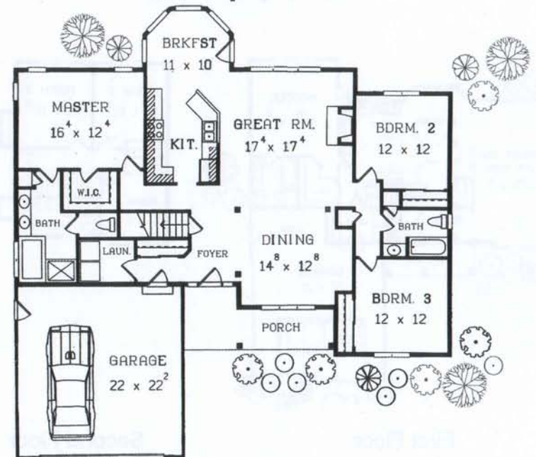
Jordyn 1817 Square Feet
