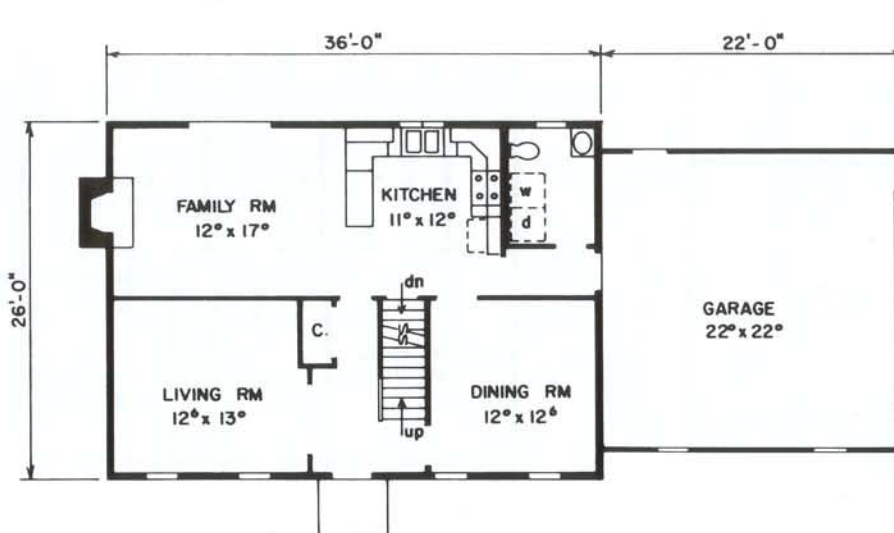
First Floor 936 Sq. Ft.
