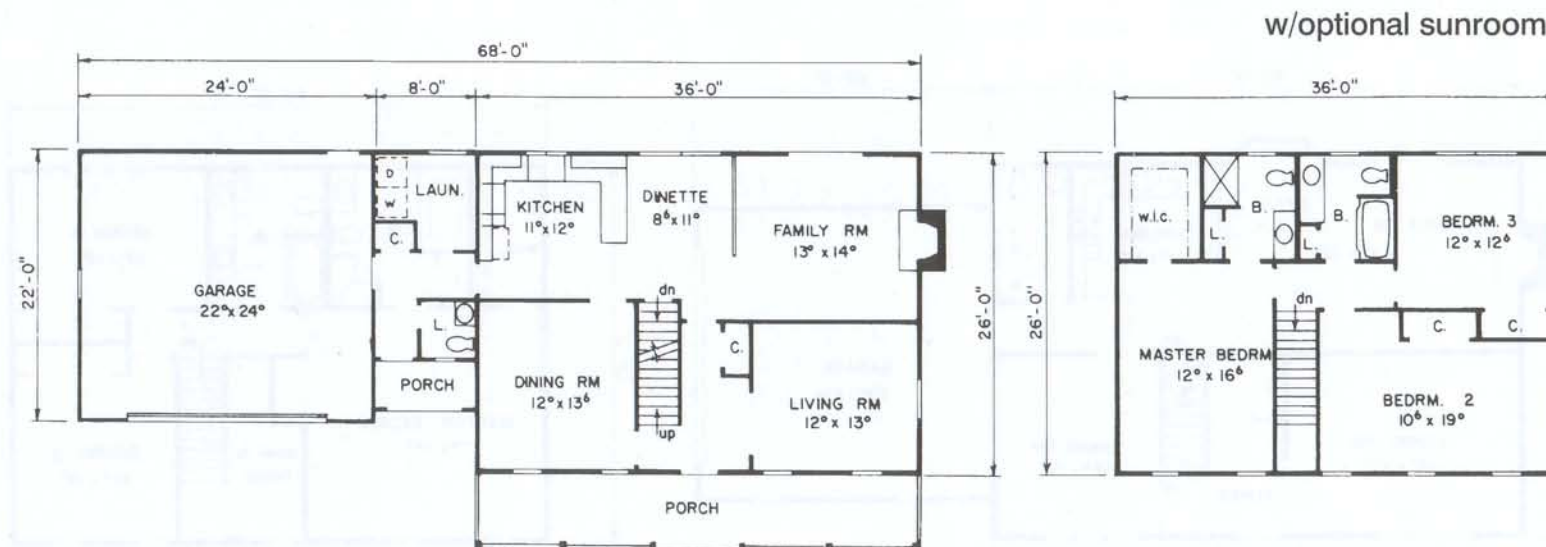
First Floor 1072 Sq. Ft.
