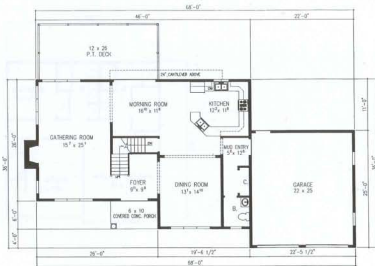
First Floor 1316 Sq. Ft.
