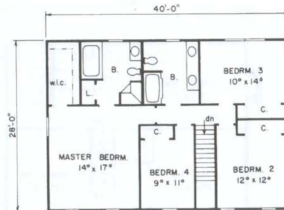
Second Floor 1120 Sq. Ft.
