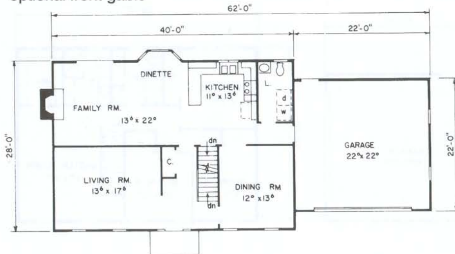
First Floor 1120 Sq. Ft.
