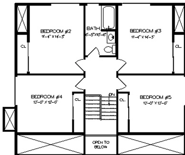
2nd FLOOR PLAN 905 SQUARE FEET
