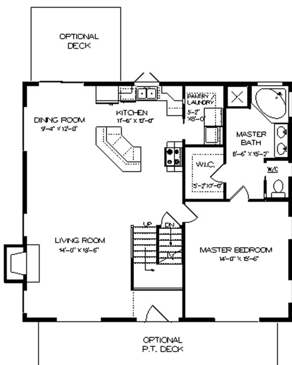
1st FLOOR PLAN 1157 SQUARE FEET
